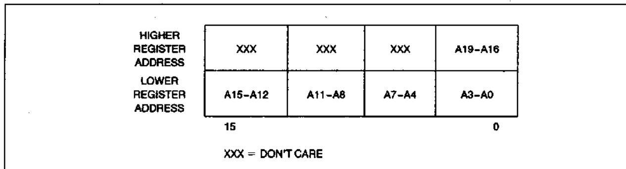
Figure 18. DMA Pointer Register Format
