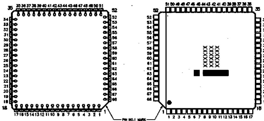
Contacts Facing Up
