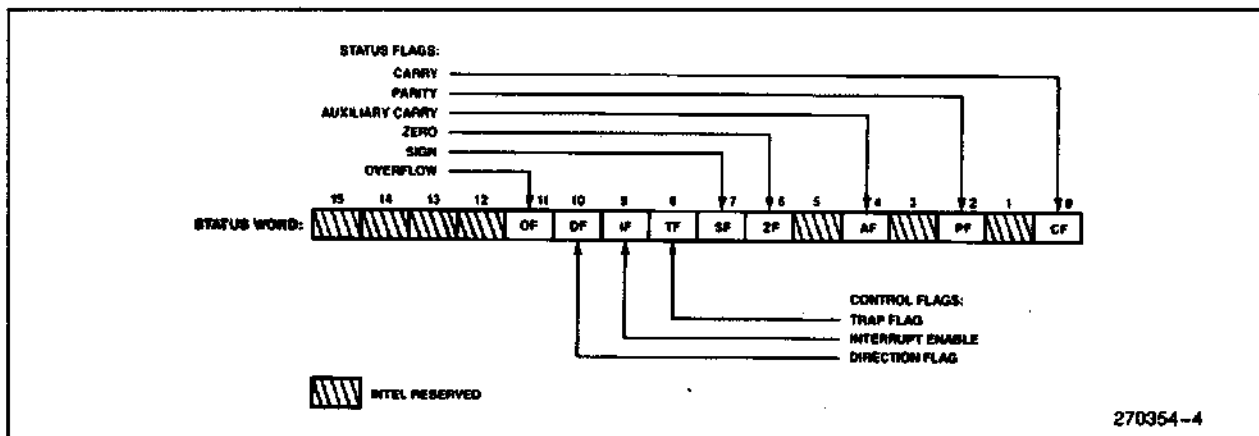
Figure 3b. Status Word Format 24-67
