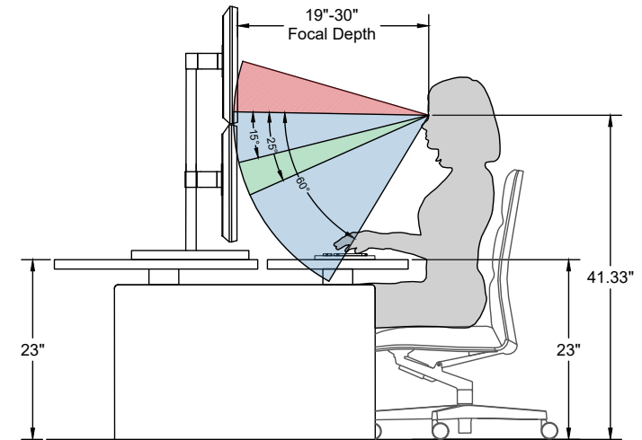
5TH PERCENTILE FEMALE (4'-11") BASED ON 24" FLAT PANEL MONITORS
