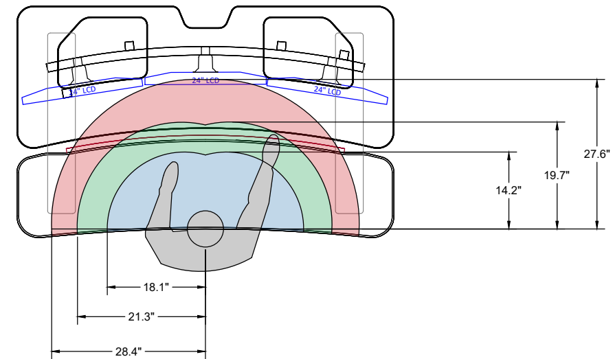
REACH ZONES FOR STRAIGHT WORKSTATION
