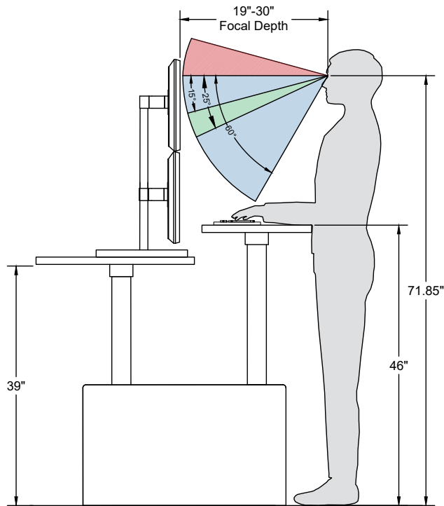
95TH PERCENTILE MALE (6'-4") BASED ON 24" FLAT PANEL MONITORS
