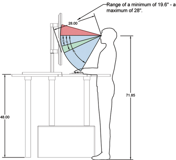
95TH PERCENTILE MALE (6' 3 1/2") BASED ON 24" FLAT PANEL MONITORS
