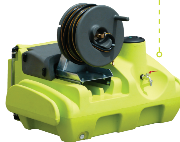
OnDeck™ 150L UTV Sprayer 7.5L/min 12v pump and 30m Reel
