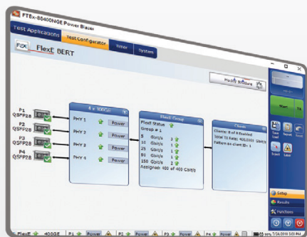
Ethernet multiclients
