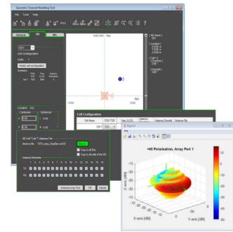
PROPSIM GCM 5G tool for scenario building.
