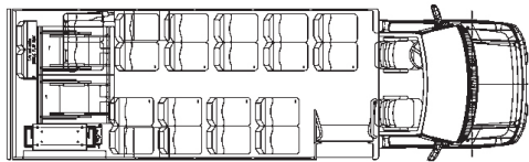
27' Spirit 22 Passenger + 2 Wheel Chair with Rear Lift
