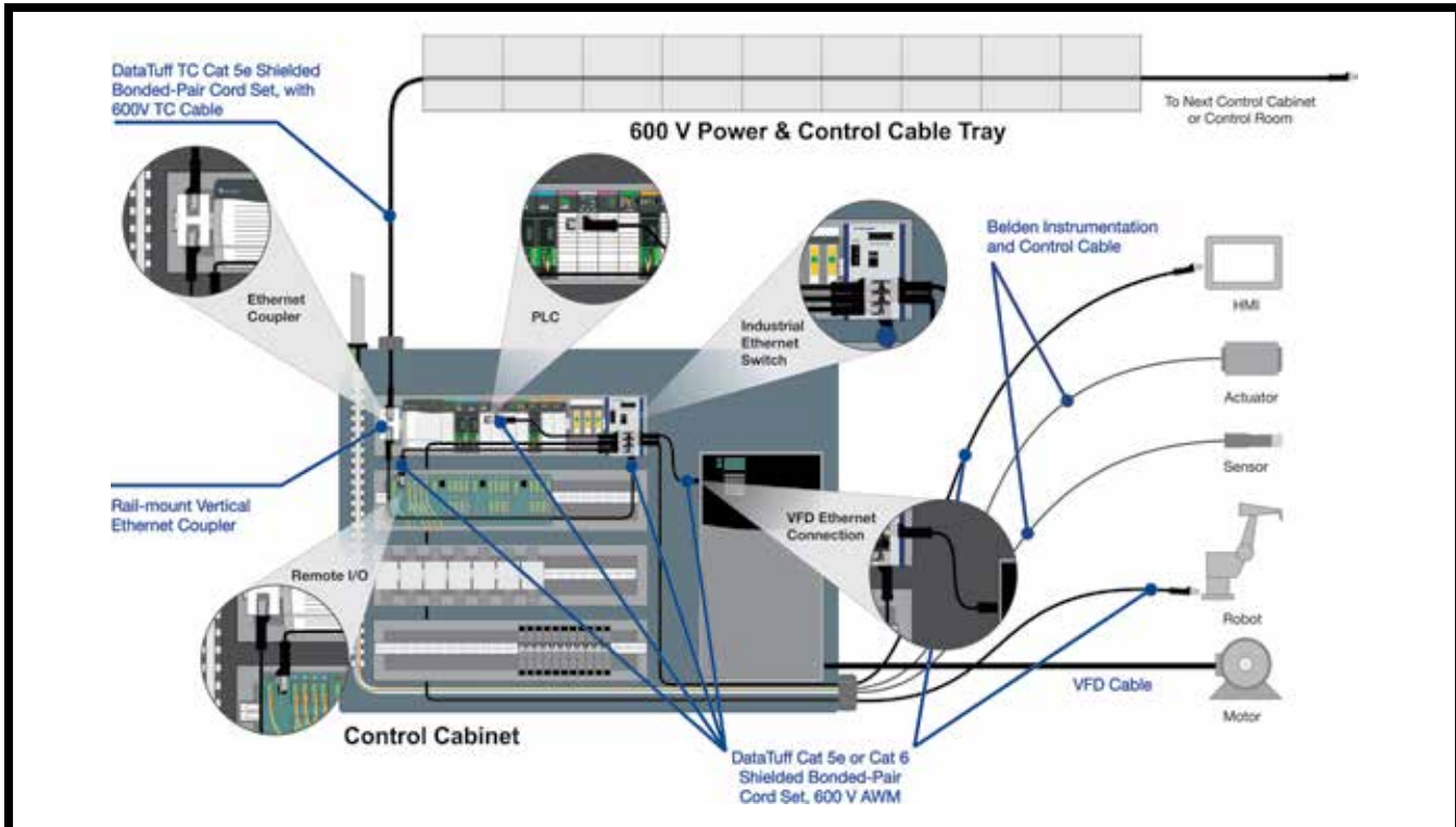
Industrial Cable - Installation Example (UL 1277 Listed, Type TC 600V Industrial Ethernet Cable)
