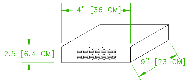
INDIVIDUAL LOCKER DIMENSIONS
