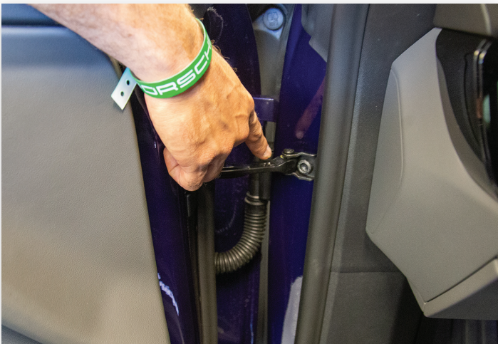
Make the 12-volt negative connection at the door check on the driver side door.
