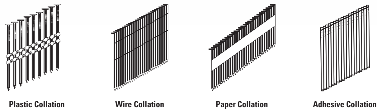
Examples of BOSTITCH® Stick Nails
