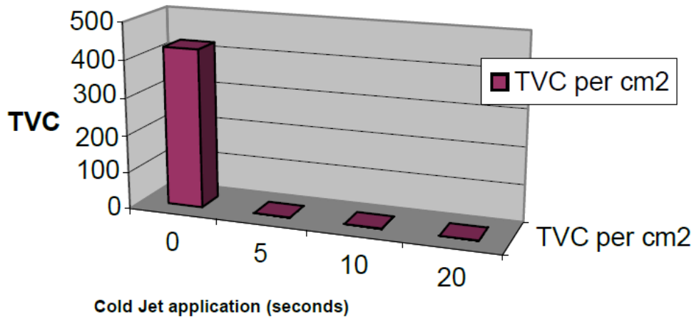
Figure 5.36 Effect of Cold Jet (PFR = 60) application on ceramic tiles on TVC L.monocytogenes
