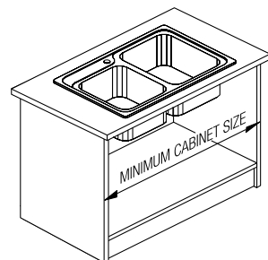
Diagram A Measure from outside edges of cabinet for minimum cabinet size.
