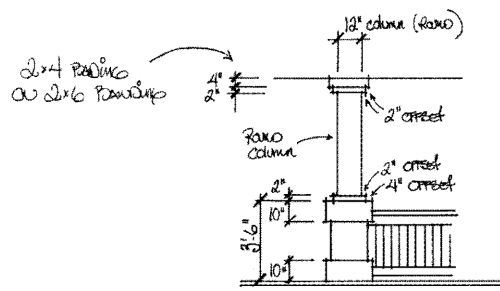
column detail
