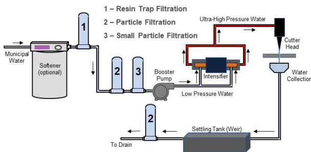
Figure 1 - Direct Feed Water System
