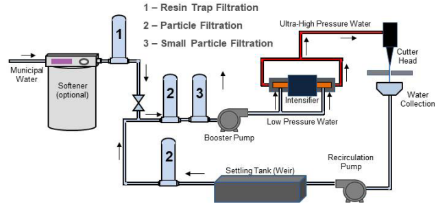
Figure 2 - Recirculating Water System
