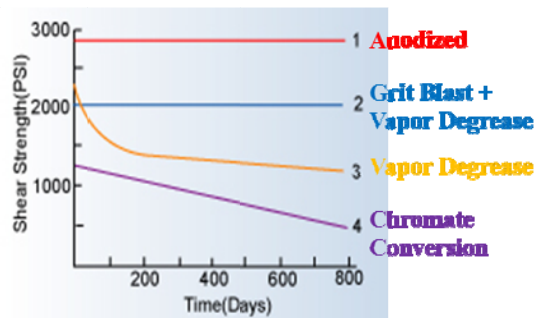
Aluminum/Epoxy Joint Strength - H2O Immersion
