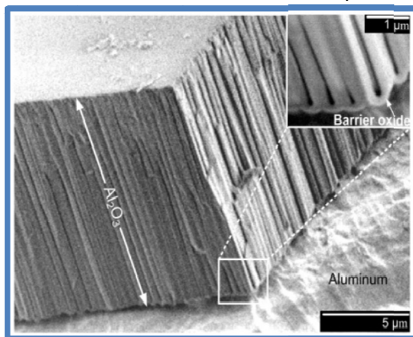
Anodized surface under an electron microscope
