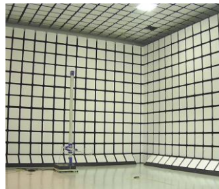
On-site Anechoic Chambers for Emission Testing
