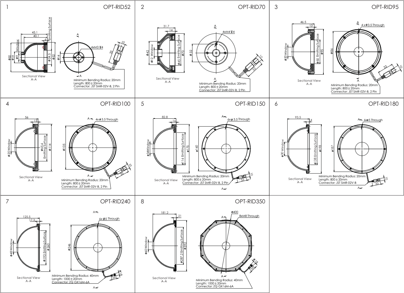
Dimensional Drawings [mm]
