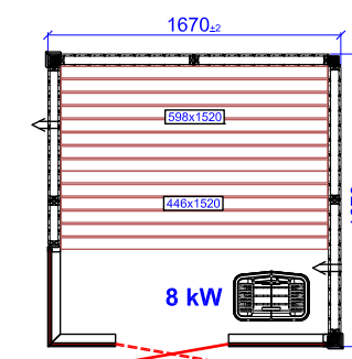
HARMONY GC LEFT 1670X1670
