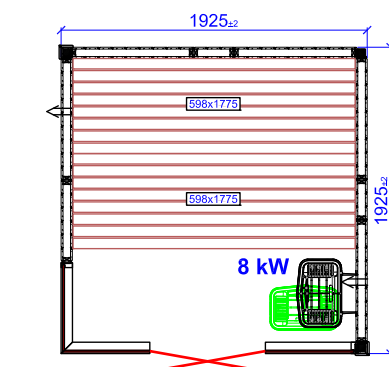
HARMONY GC LEFT 1925X1925
