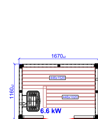
HARMONY GF 1670X1160
