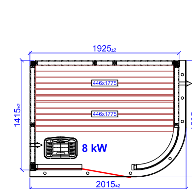
HARMONY GC ROUND 1925X1415
