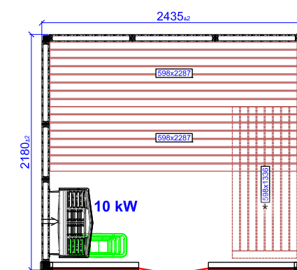
HARMONY GF 2435X2180 *Third bench with bench support needs to be ordered as special.
