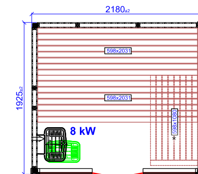
HARMONY GF 2180X1925 *Third bench with bench support needs to be ordered as special.
