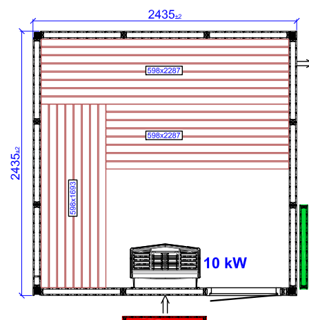
HARMONY SQ 2435X2435
