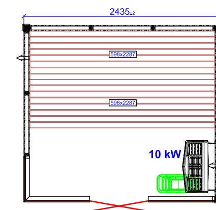
HARMONY GC LEFT 2435X2180
