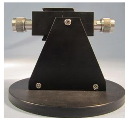
Fig 2. Test fixture for SE measurements at f= 1.5 - 10 GHz.
