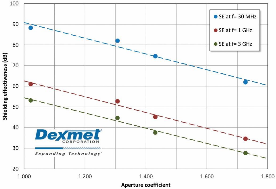
Fig 6. Linear dependence of SE on aperture coefficient for four (4) copper EMFs from Fig 5.
