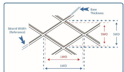
Fig 4. Dimensions of expanded metal foils.
