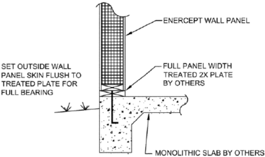
FIGURE 4—TYPICAL WALL TO MONOLITHIC SLAB
