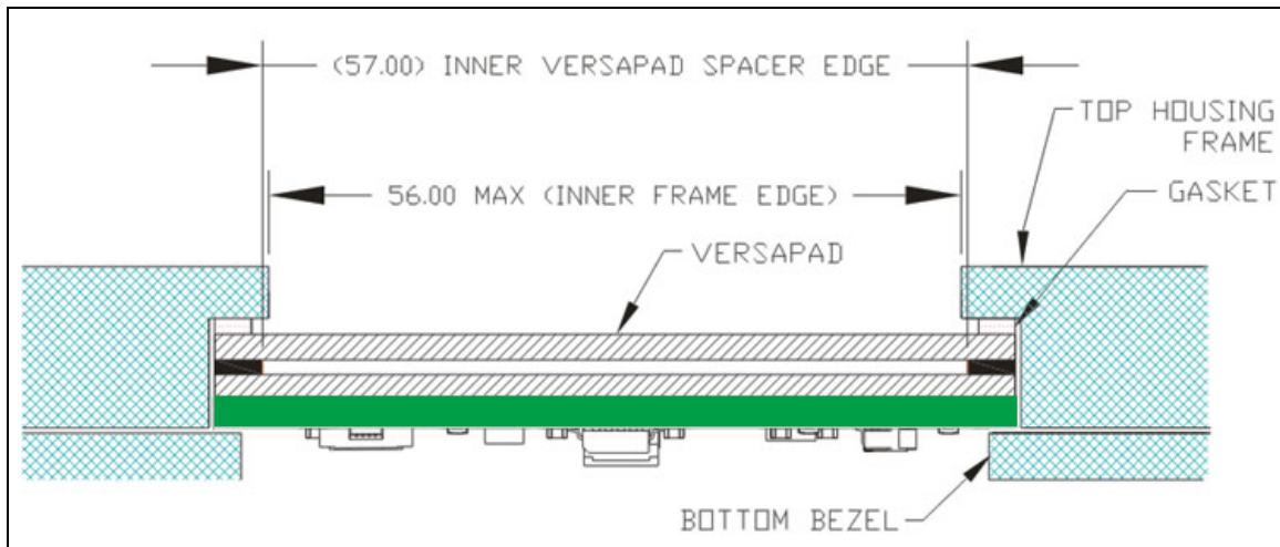
Figure 6: Side view of bottom side mounting. Drawing is not to scale
