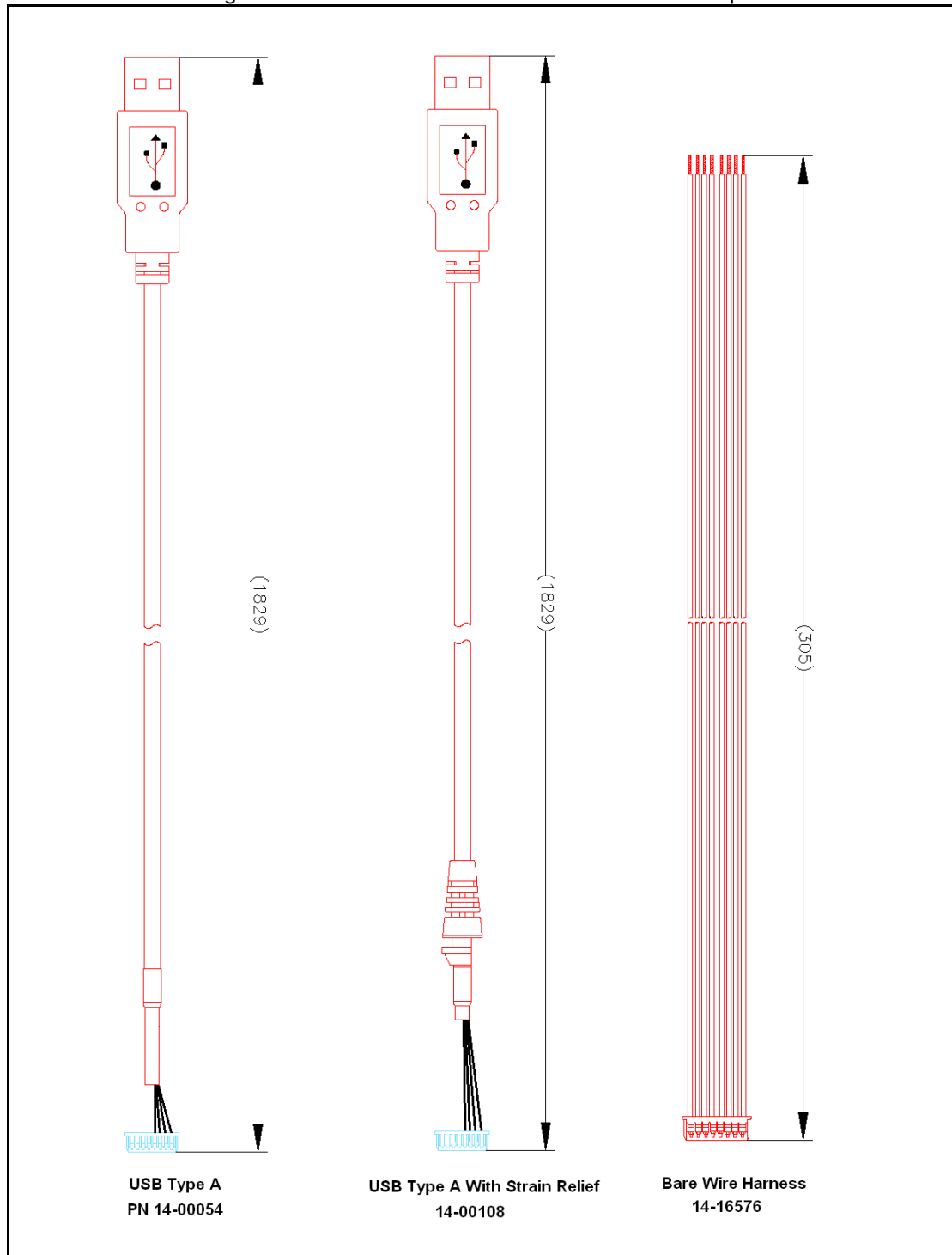
Figure 11: USB VersaPad Standard Cable Options
