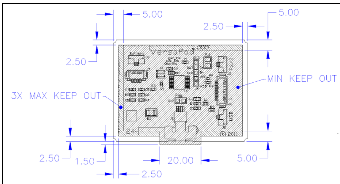
Figure 8: Mounting Bracket & Keep out Area. Drawing is not to scale
