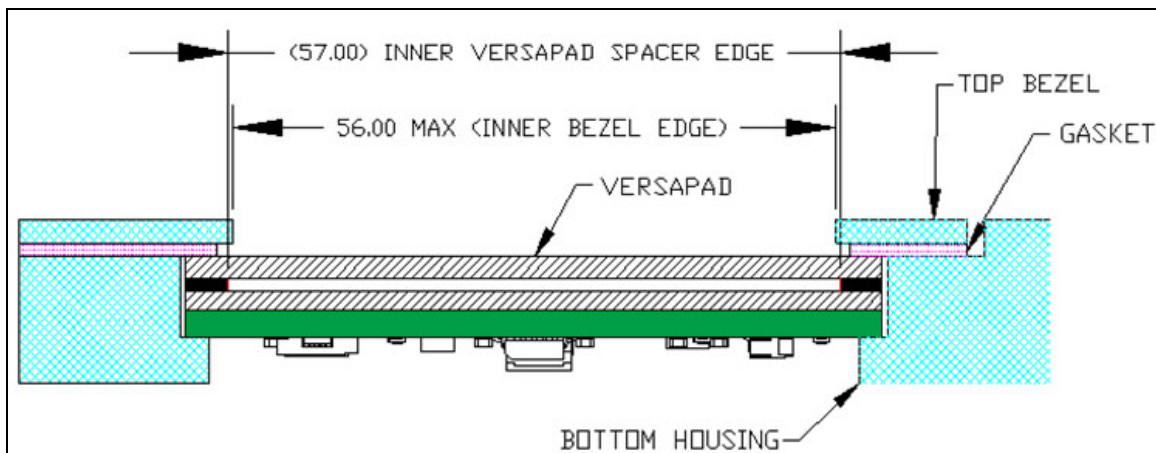
Figure 7: Side view of top side mounting. Drawing is not to scale
