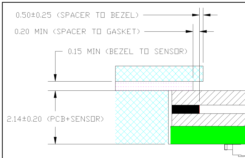
Figure 5: Critical capture dimensions. Drawing is not to scale.
