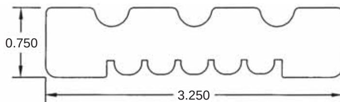
3 1/4" Fluted & Reeded Case BL67
