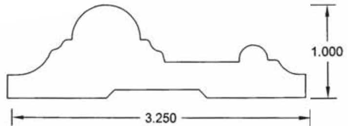
3 1/4" Chair Rail BL56
