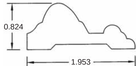
2" Panel Mold BL52
