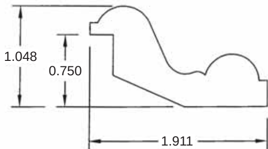
3/4" Raised Panel Mold BL55
