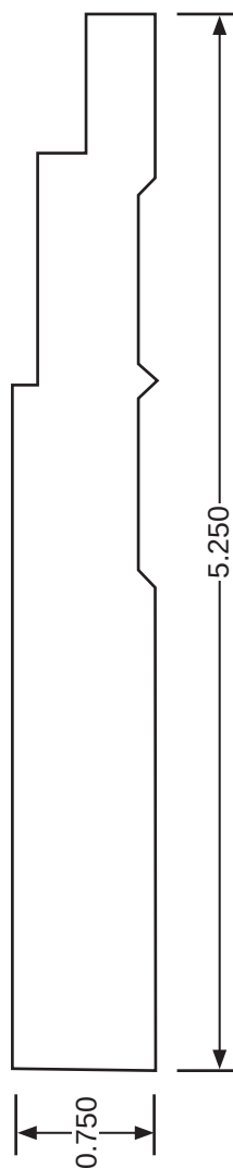
2 Step Base BL413
