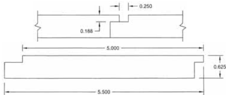
5 1/2" Shiplap BL411
