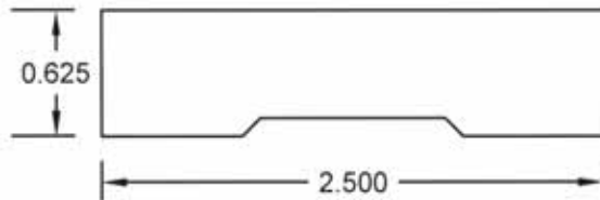
2 1/2" Contemporary Case BL409
