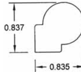
Staff Bead BL63
