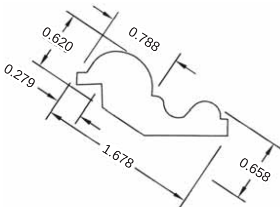
1/2" Raised Panel Mold BL54
