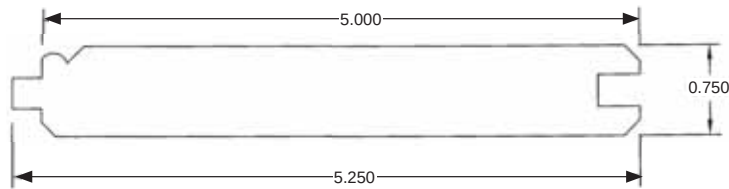
5" T&G V-Groove and Beadboard BL60
