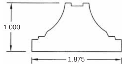
1 7/8" Panel Mold BL51
