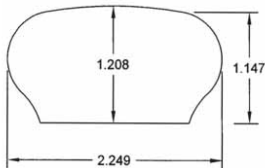
2 1/4" Handrail BL65
