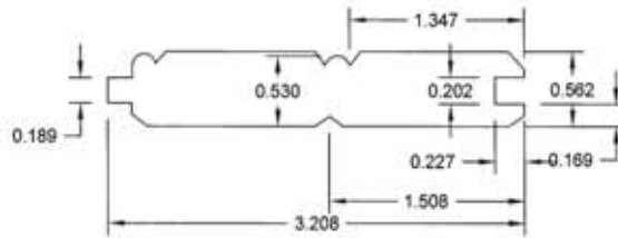
Fir T&G Bead and V-Groove BL58
