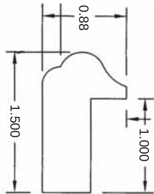
Wainscot Panel Cap BL64
