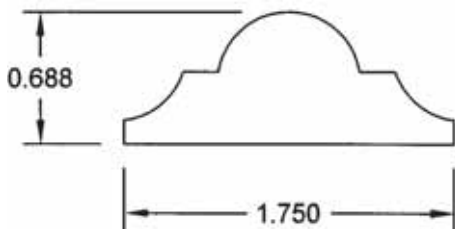
1 3/4" Bead Panel Mold BL48
