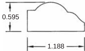
Neck Mold BL46
