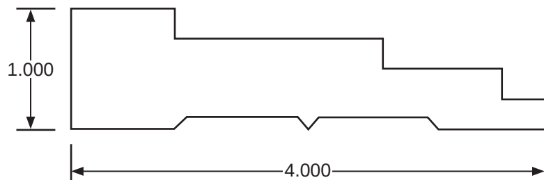
3 Step Case BL412
