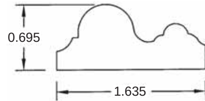
1 5/8" Panel Mold BL50
