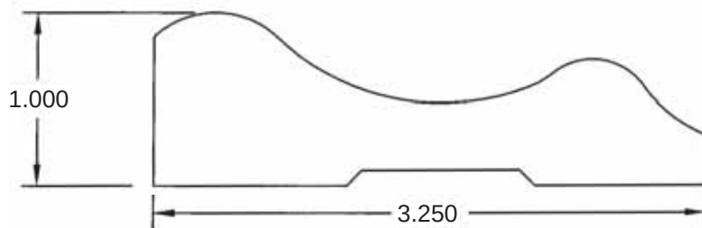
3 1/4" Ovalo Case BL66
