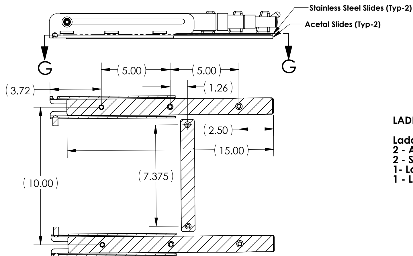
SECTION G-G
