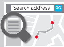
ADDRESS VERIFICATION
