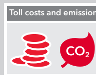
ROUTE CALCULATION
