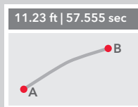
DISTANCE CALCULATION
