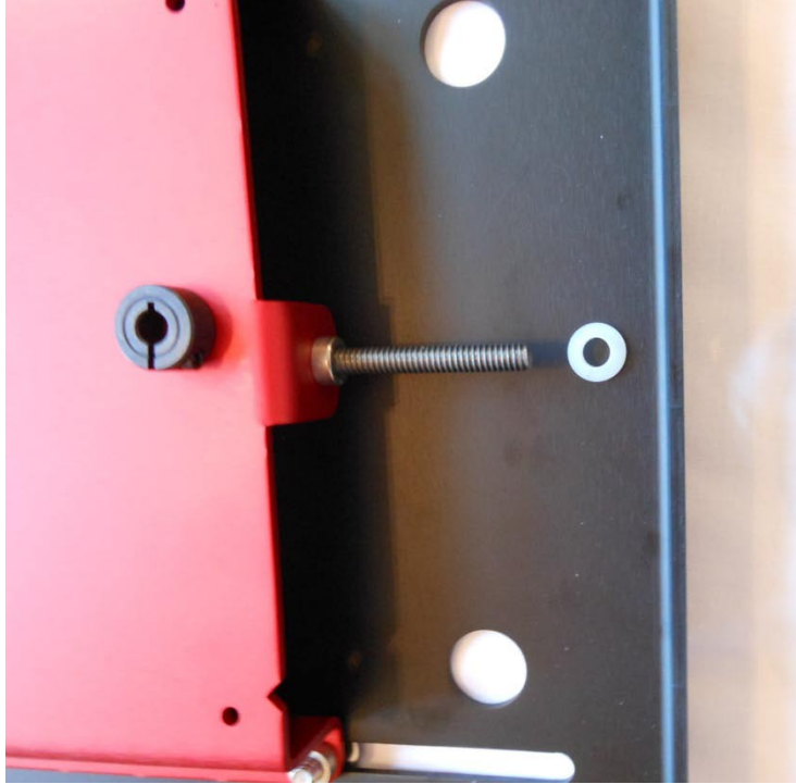
Original shaft collar shown - Alternate aluminum collar is also OK.
