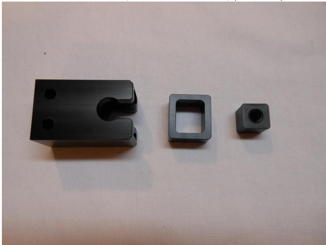
Z Drive: Mount ZD-01, Frame ZD-02 & Nut ZD-03, (Black Delrin)
