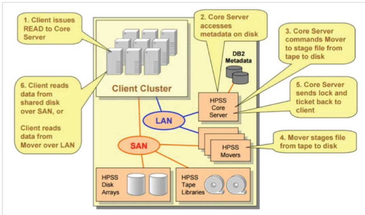
Figure 1 – HPSS Architecture
