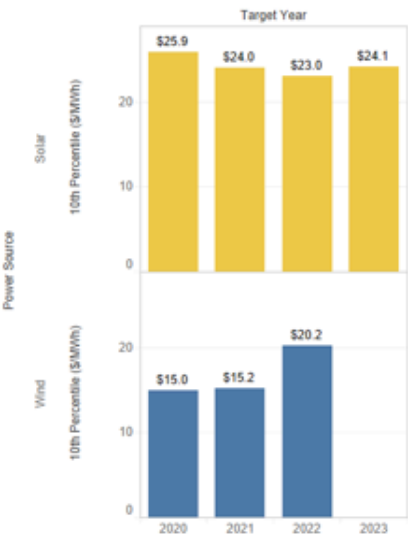
10th Percentile PPA Prices by COD
