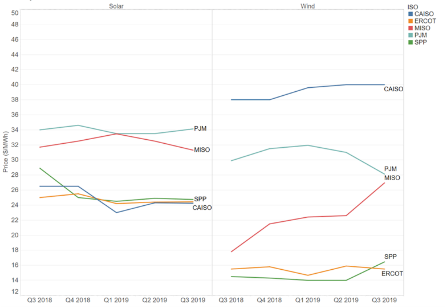
Quarterly ISO Price Indices- P25
