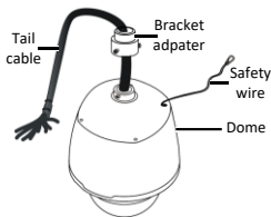
Figure 1 Camera components
