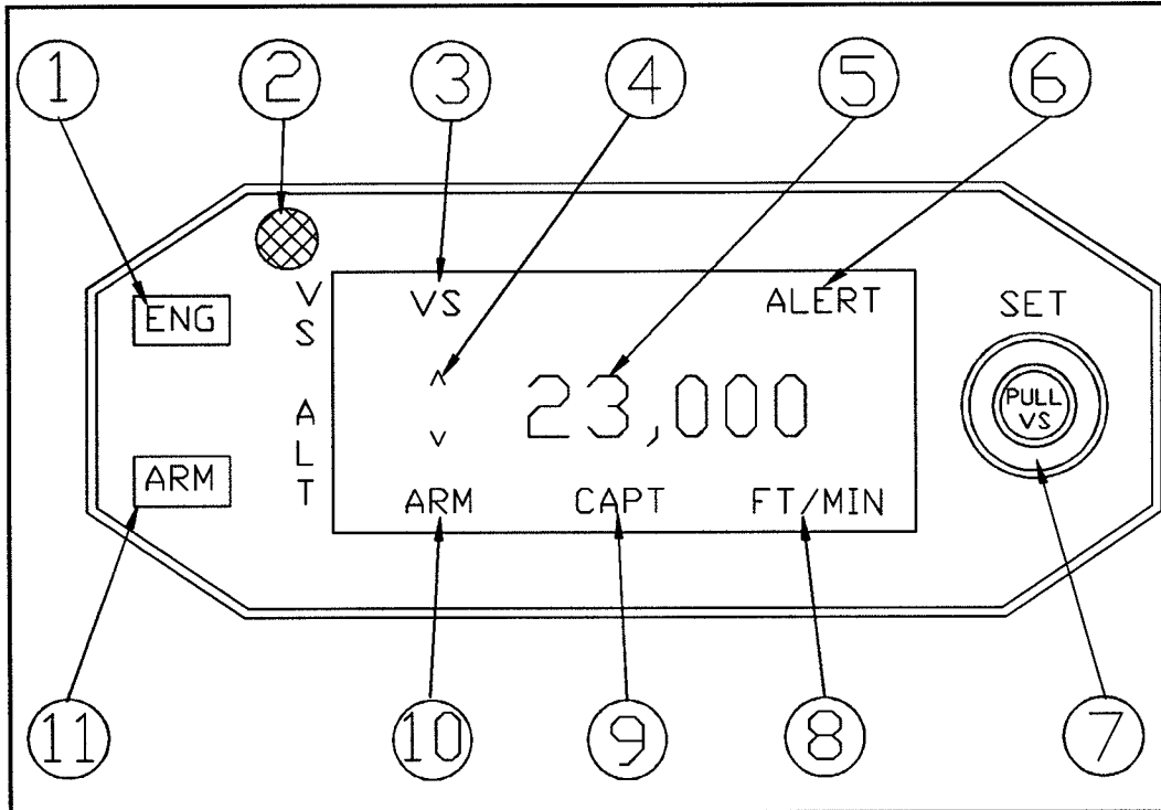
FIGURE 1 - KAS 297B VERTICAL SPEED AND ALTITUDE SELECTOR
