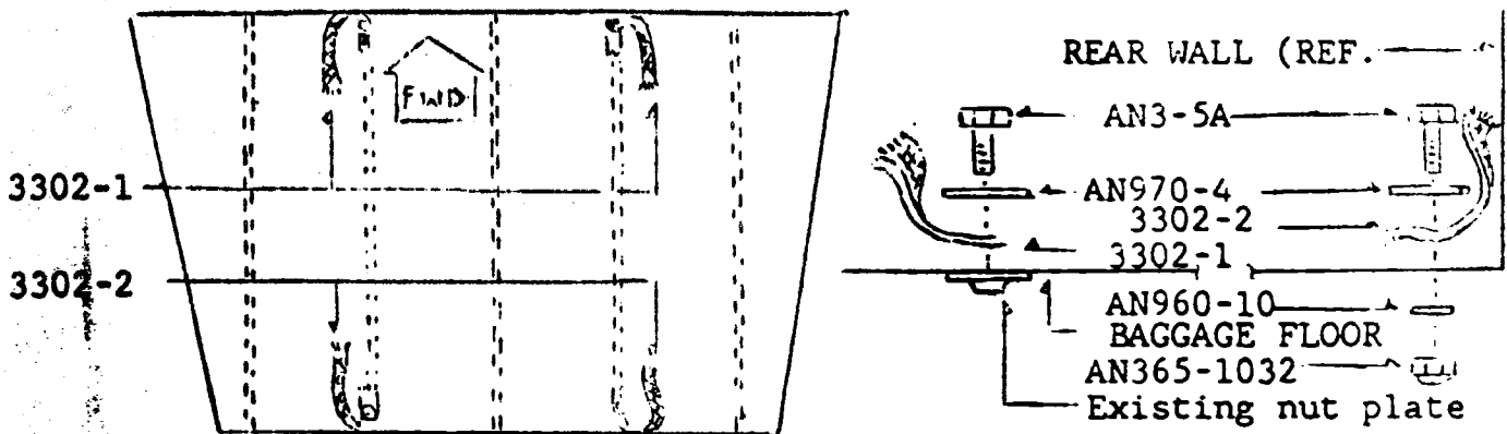
VIEW LKG DOWN AT BAG FLOOR FIG. 1
