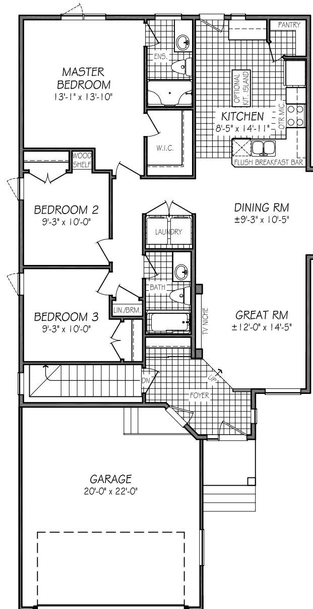
MAIN FLOOR PLAN 1380 SQ. FT.
