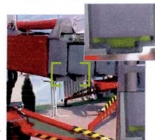
TIVAR® Ceram P® performs well as a slide panel in telescoping booms. Outstanding abrasion resistance adds to the wear-life of the pad.
