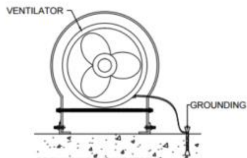
GROUNDING CONNECTION DIAGRAM
