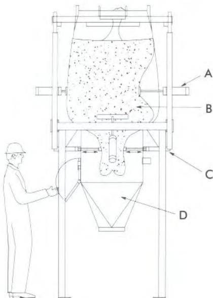
A. Side Massagers B. Base Massagers C. Spout closure bars D. Discharge chute
