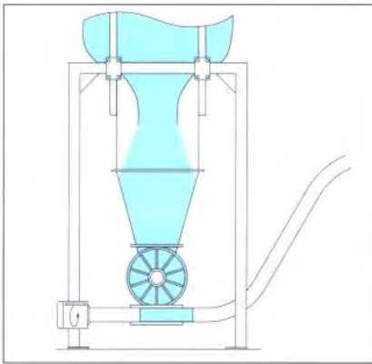
Pneumatic conveyor
