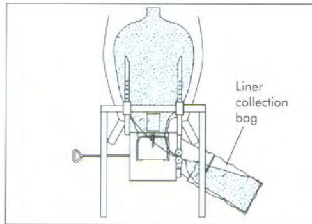
Liner removal and tensioning mechanism.
