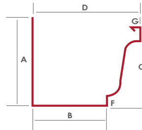
K-Style Gutter Design
