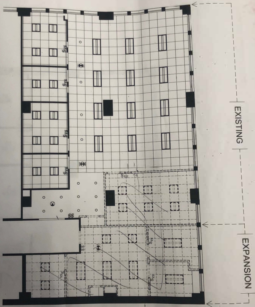
2 CEILING DEMOLITION PLAN SCALE: 1/8" = 1'-0"
