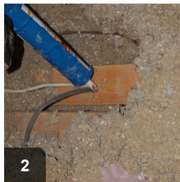
Use caulk or foam (approved by local code) to seal wiring penetrations through top plate
