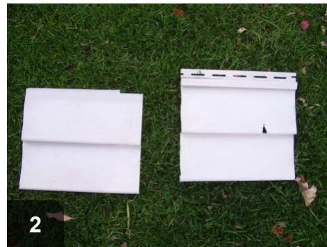
Use siding that matches the existing material's contour, texture, and color
