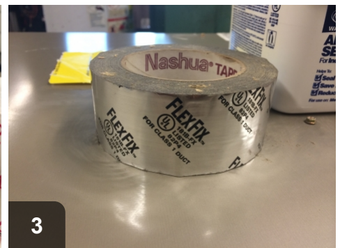
3 Use tape to assemble joints, then coat with at least 2mm of mastic
