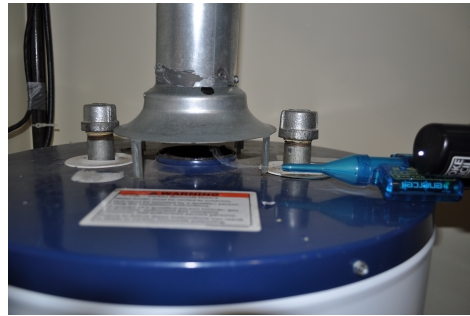
Complete spillage test using chemical smoke pencil
