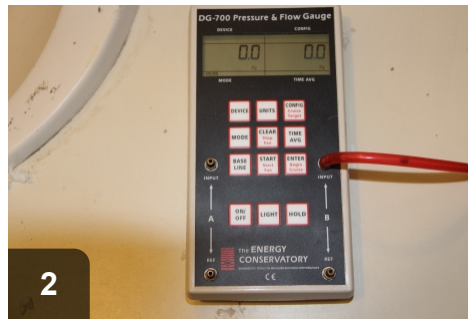
2 Attach hose to the manometer set to PR/PR.
