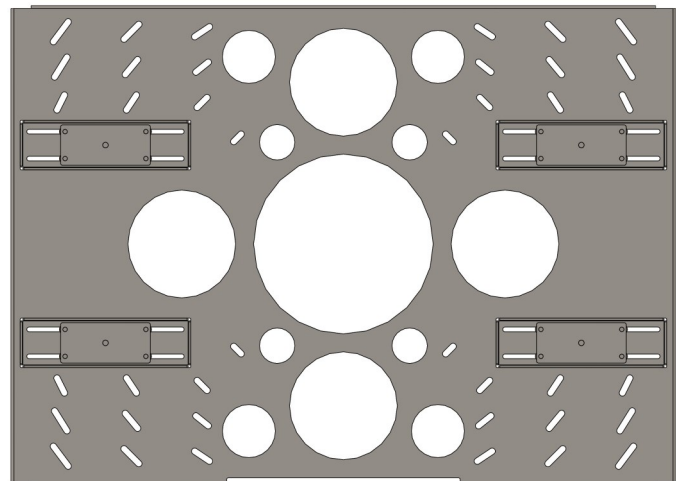
Wallmate 32MAX Horizontal Shift VESA Plate
