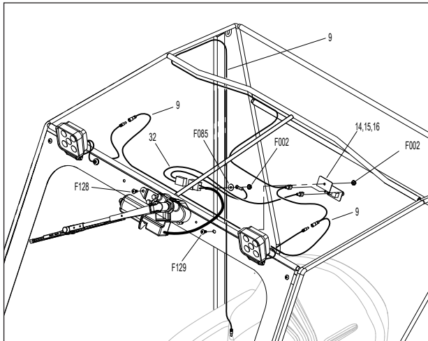
Route Wiring for Windshield Wiper Motor, Headlights, and Windshield Wiper Toggle Switch
