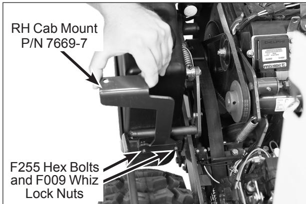
RH Cab Mount Installation
