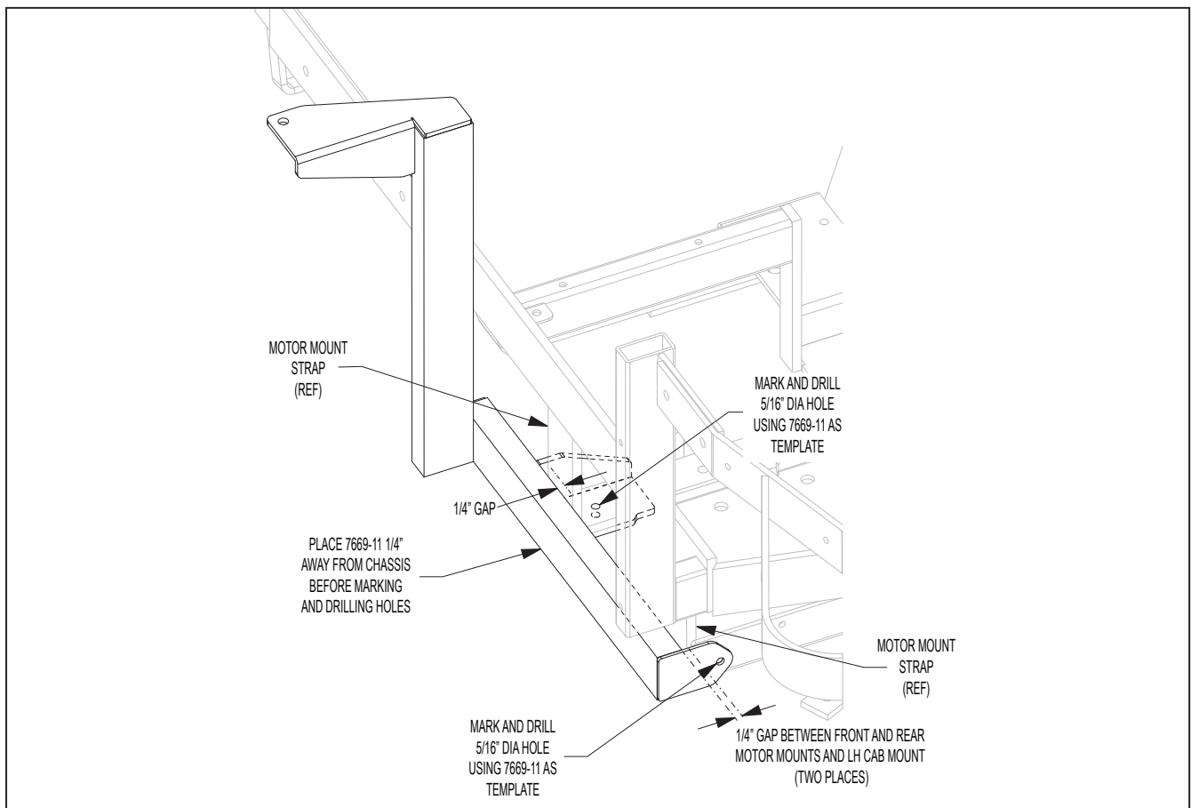
Motor Mount Strap and LH Cab Mount Gap (1/4 in.)
