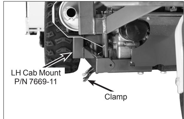
LH Cab Mount Installation
