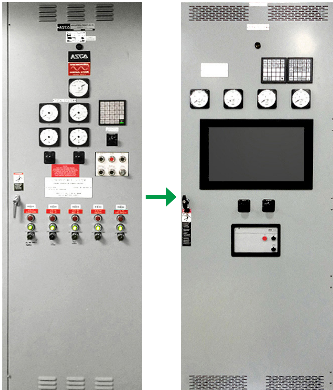
Figure 2: The legacy Master Control Section at left was upgraded as shown at right. The upgrades included added annunciation, a large-screen HMI, and replacement of the legacy Master 90-30 controller with a new Rx3i controller.
