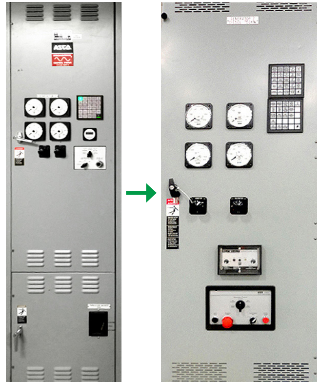
Figure 3: At the same site, a legacy Generator Control Section at left was upgraded with added annunciation and its Generator 90-30 PLC was replaced with the Versamax unit.
