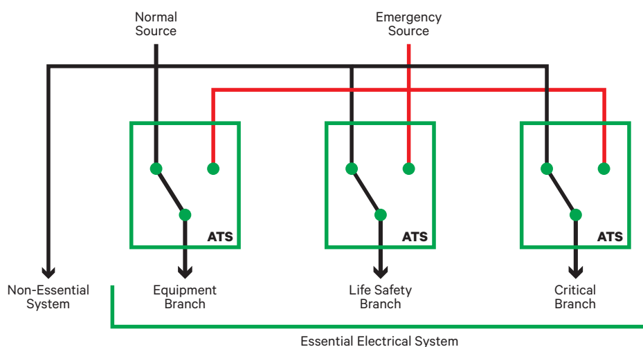
Figure 1: NEC Essential System Configuration
