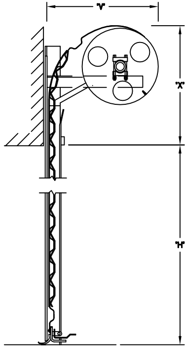
SECTION-A-A
