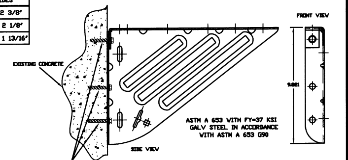
LH DOOR MOUNTING BRACKET DETAIL
