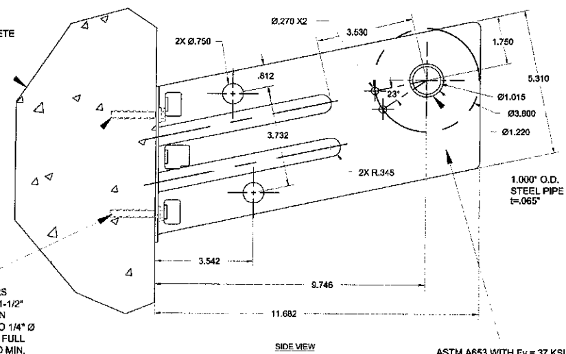
DOOR MOUNTING BRACKET DETAIL
