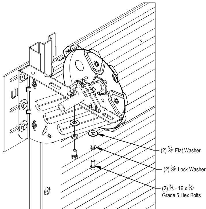
FIGURE 16: TENSIONER END
