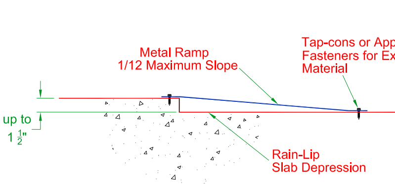
ADA RAMP Section View
