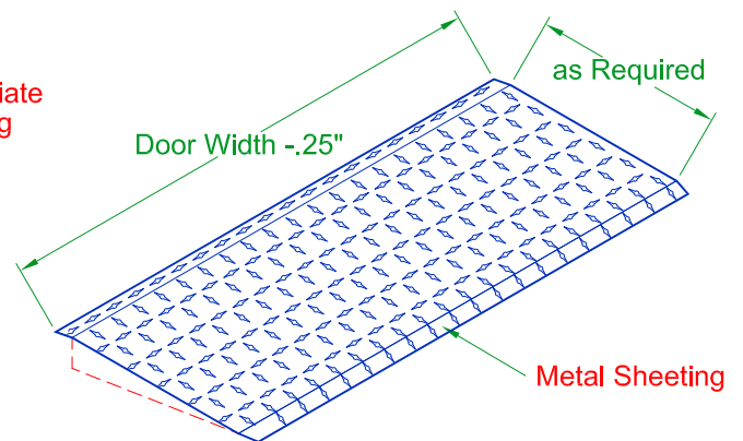
ADA RAMP Isometric View
