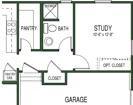
OPTION #4 - OPTIONAL WALK-IN PANTRY AND OPTIONAL SHOWER IN BATHROOM (REQUIRES 2nd FLOOR OR BASEMENT LAUNDRY)
