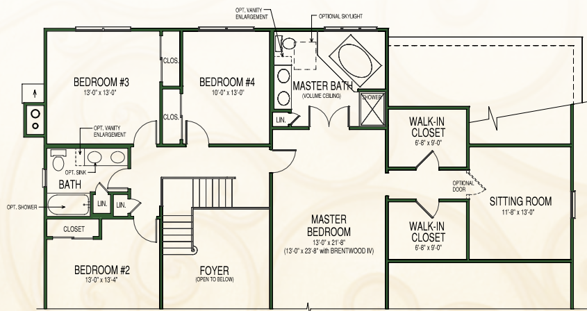
OPTIONAL 2'-0" REAR CANTILEVER WITH DUAL SINKS IN MAIN BATH (SHOWING BRENTWOOD IV)
