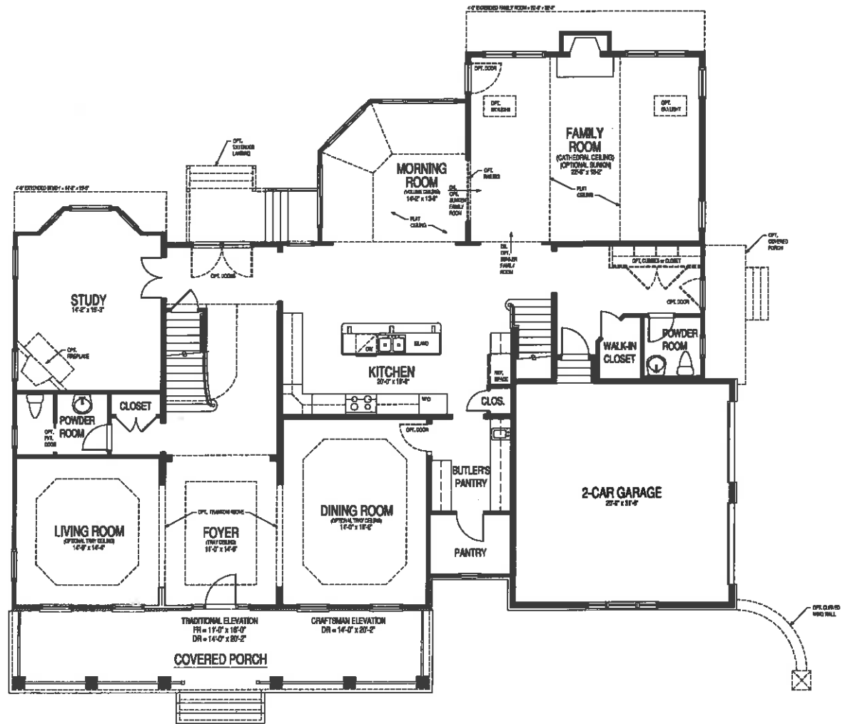
FIRST FLOOR
