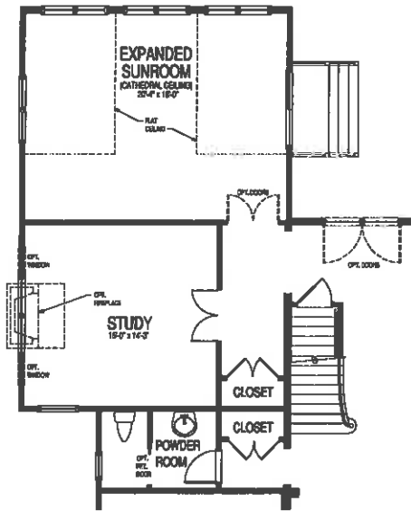
OPTIONAL EXPANDED SUNROOM w/ STUDY
