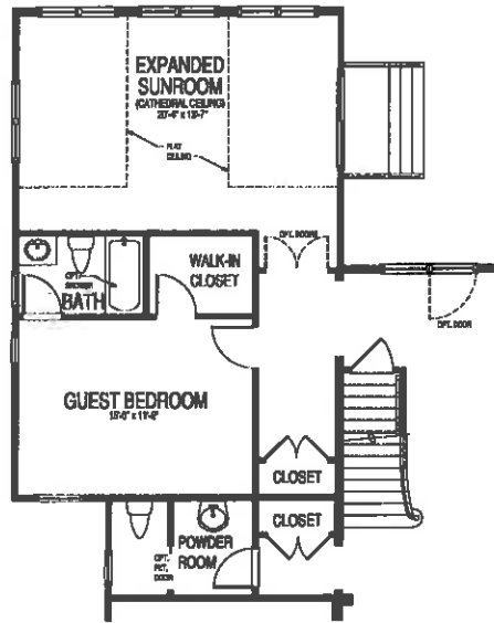
OPTIONAL EXPANDED SUNROOM w/ GUEST BEDROOM
