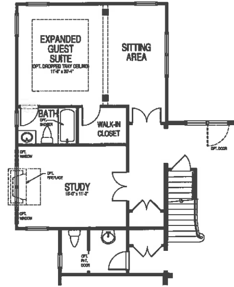
OPTIONAL EXPANDED GUEST SUITE w/ SITTING AREA AND STUDY
