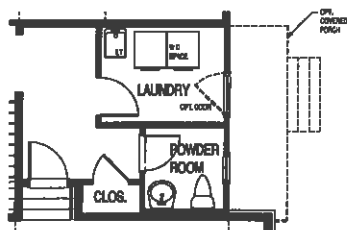
OPTIONAL FIRST FLOOR LAUNDRY ROOM
